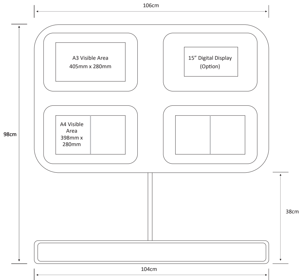
Claralight 4 Panel Freestanding Display Dimensions
