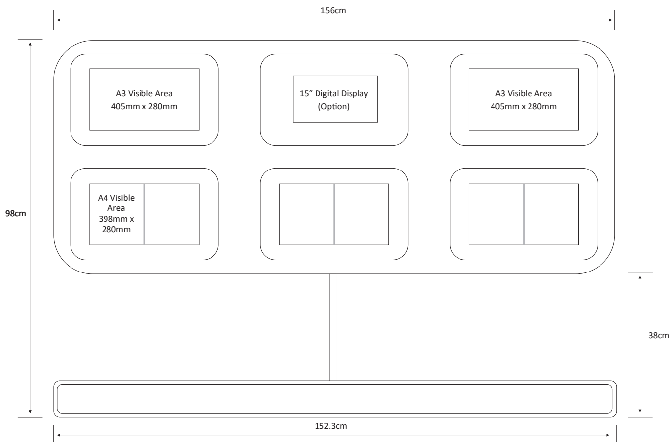
Claralight 6 Panel Freestanding Display Dimensions
