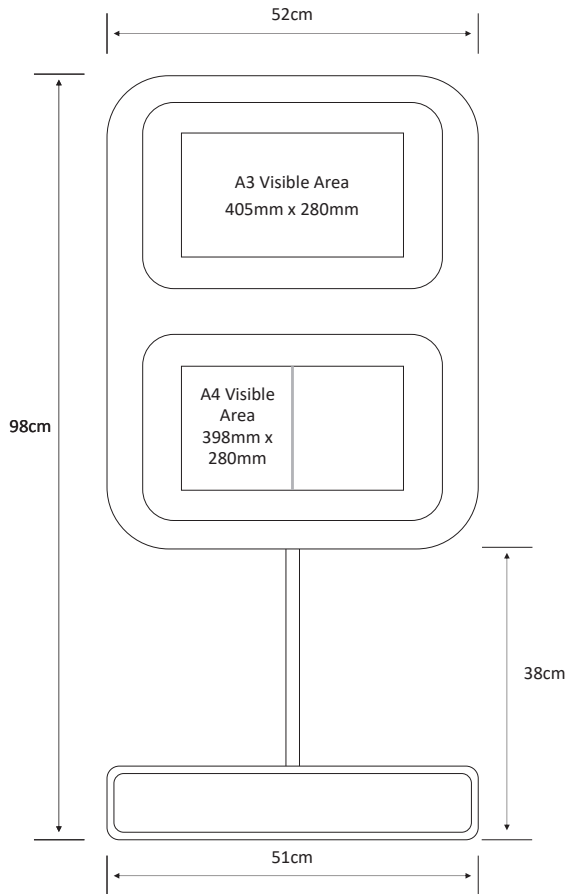
Claralight 2 Panel Freestanding Display Dimensions
